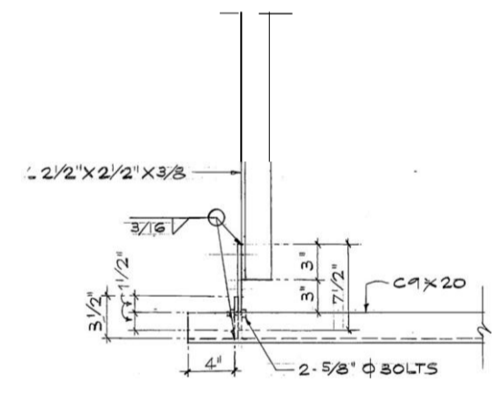
DETAIL E
